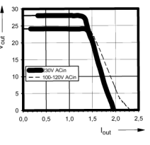
Fig. 1: Vout vs. Iout (min.)
