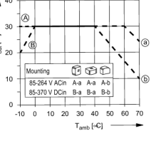
Fig. 2: Derating
